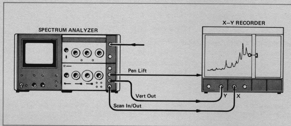
Figure 13. X-Y Recording.
