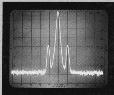
Figure 6. Single Exposure.
