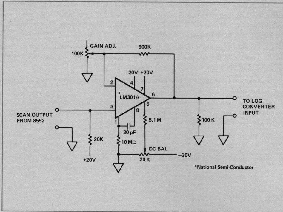
Example circuit for Amplifier 1 shown in Figure 23.
